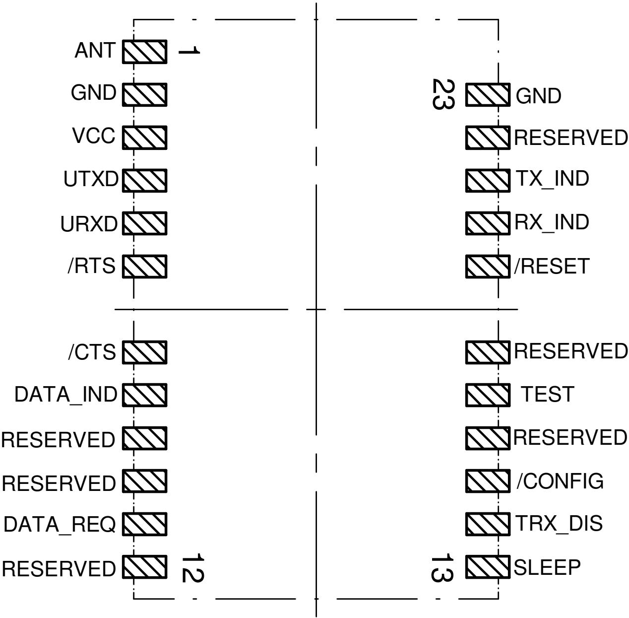
Figure 2: Pinout
